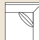
3661 Corner Chair Overall: H 36 W 38 D 38 Seating: H 16 W 21 D 21 Seat Height: 20 Arm Height: 26 Pillows: 2 P21
