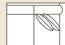
3673 RAF One Arm Loveseat Overall: H 36 W 54 D 38 Seating: H 16 W 45 D 21 Seat Height: 20 Arm Height: 26 Pillows: 2 P21
