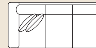
3652 LAF One Arm Sofa Overall: H 36 W 77 D 38 Seating: H 16 W 68 D 21 Seat Height: 20 Arm Height: 26 Pillows: 2 P21
