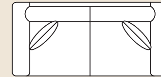
3675 Studio Sofa Overall: H 36 W 79 D 38 Seating: H 16 W 61 D 21 Seat Height: 20 Arm Height: 26 Pillows: 2 P21
