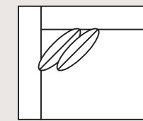
9012 LAF One Arm Chair 9013 RAF One Arm Chair Overall: H 37 W 48 D 42 Seating: H 17 W 41 D 27 Seat Height: 20 Arm Height: 25 Pillows: 2 P21
