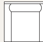
8901 Chair Overall: H 36 W 42 D 40 Seating: H 17 W 30 D 24 Seat Height: 19 Arm Height: 25
