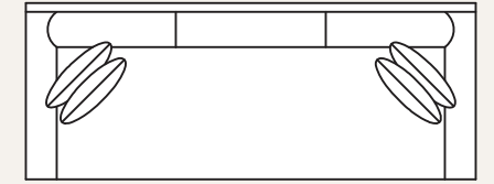
8950 Bench Cushion Sofa Overall: H 36 W 93 D 40 Seating: H 17 W 81 D 24 Seat Height: 19 Arm Height: 25 Pillows: 4 P21
