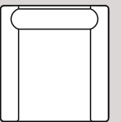
3401 Chair Overall: H 39 W 39 D 41 Seating: H 18 W 26 D 23 Seat Height: 21 Arm Height: 26
